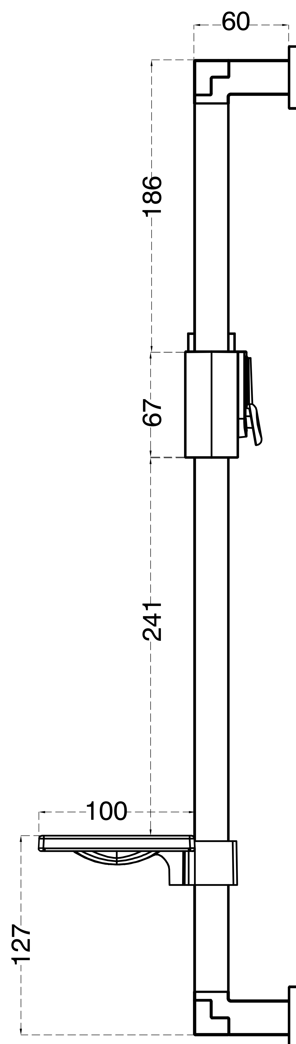
SIDE ELEVATION
