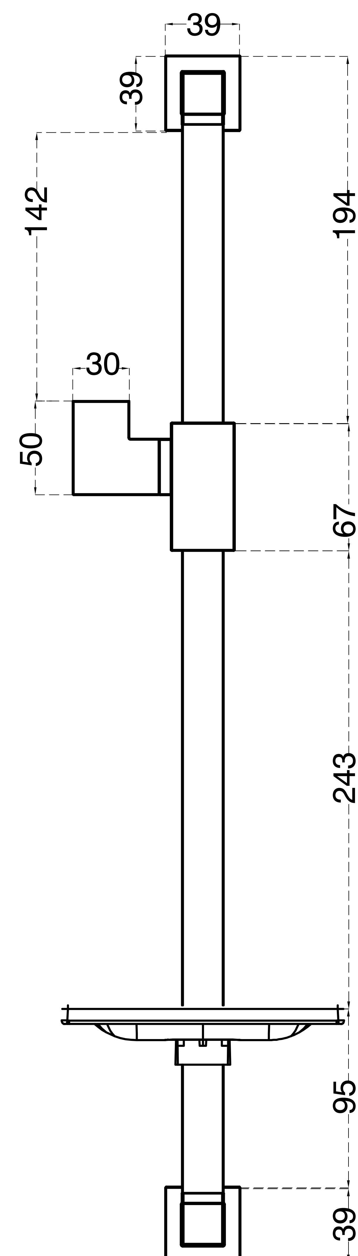
FRONT ELEVATION
